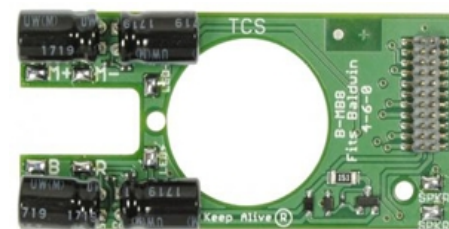
B-MB8 Motherboard 2.16 x 1.03 x 0.29 inches
